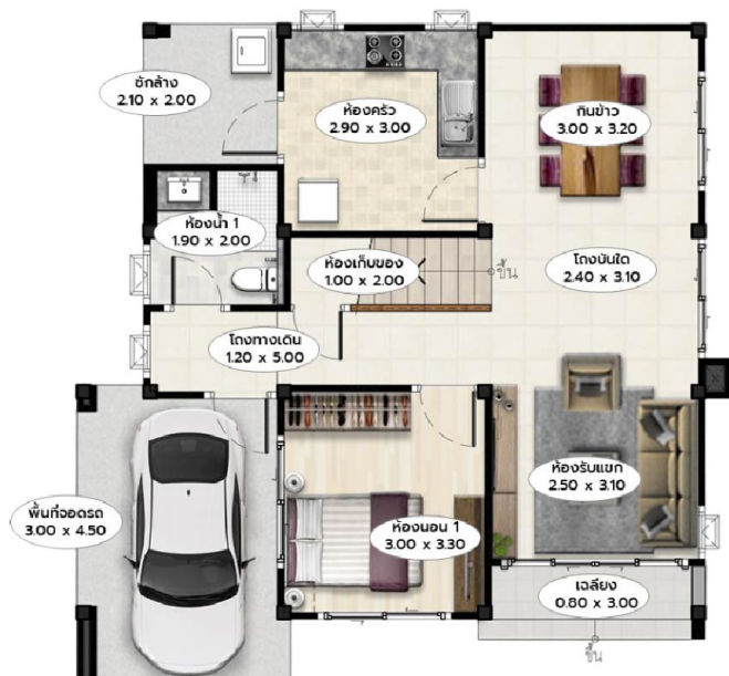
Floor Plan 1st FLOOR
