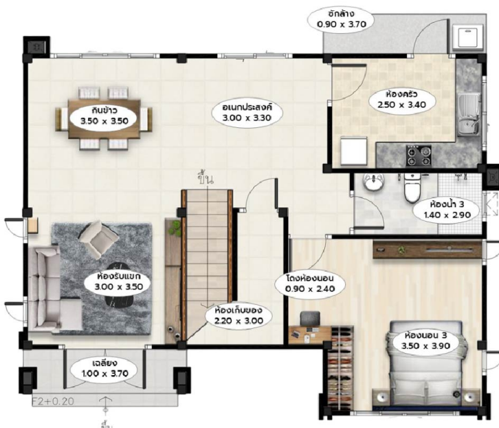
Floor Plan 1st FLOOR
