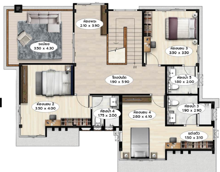
Floor Plan 2nd FLOOR
