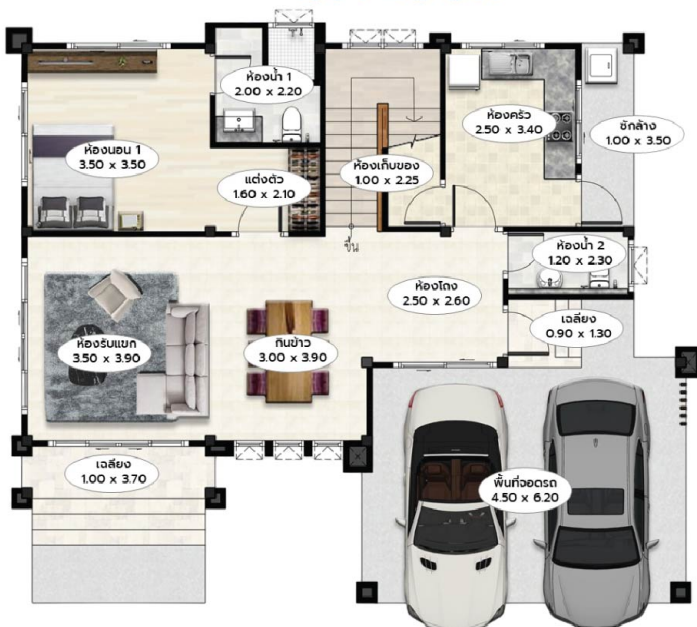
Floor Plan 1st FLOOR
