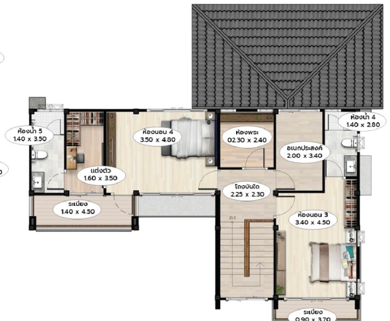
Floor Plan 2nd FLOOR
